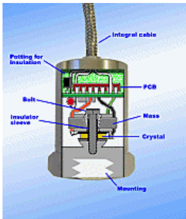
Fig 2: Transducer Construction
